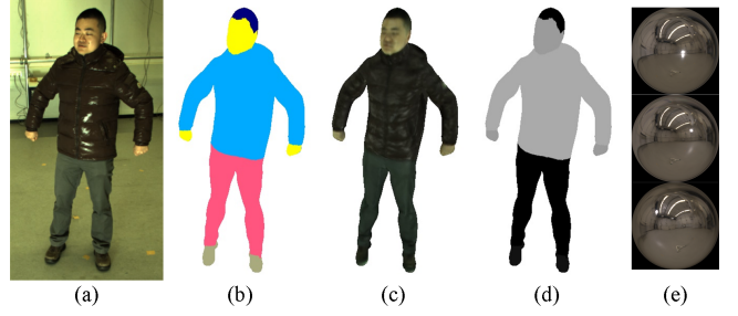
Figure 3: Reflectance estimation: (a) input image, (b) material segmentation, (c) estimated spatially varying diffuse albedo, (d) estimated per-segment specular albedo, (e) the light probe images.
